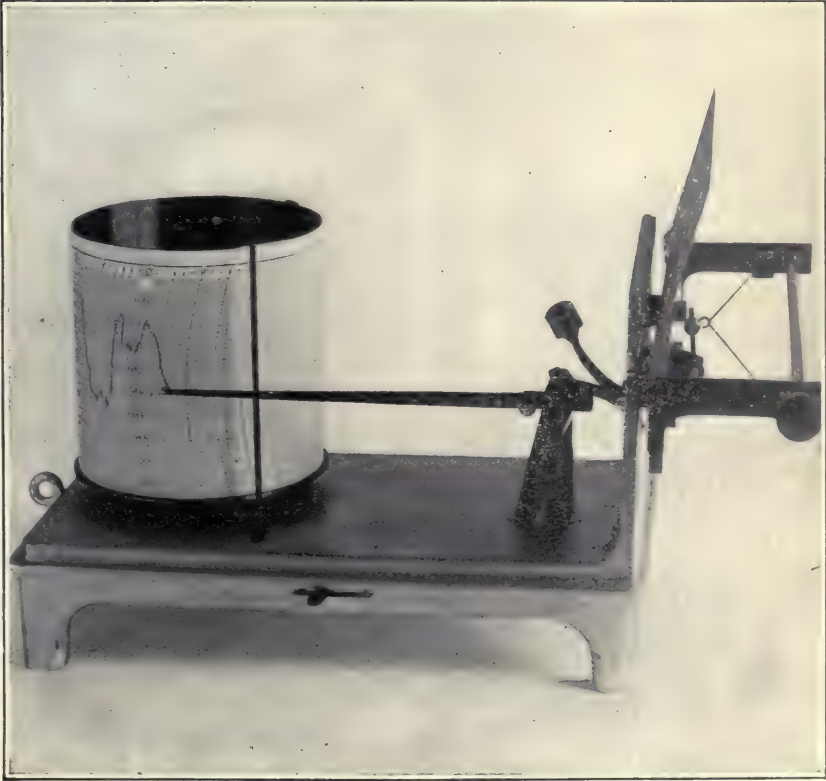
FIGURE 13. Richard's Hygrograph.
